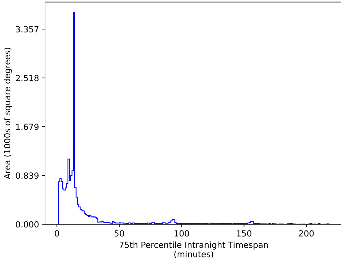
too_elab_r16_d3_gz_v3.4_10yrs WFD i band: 75th Percentile Intranight Timespan
