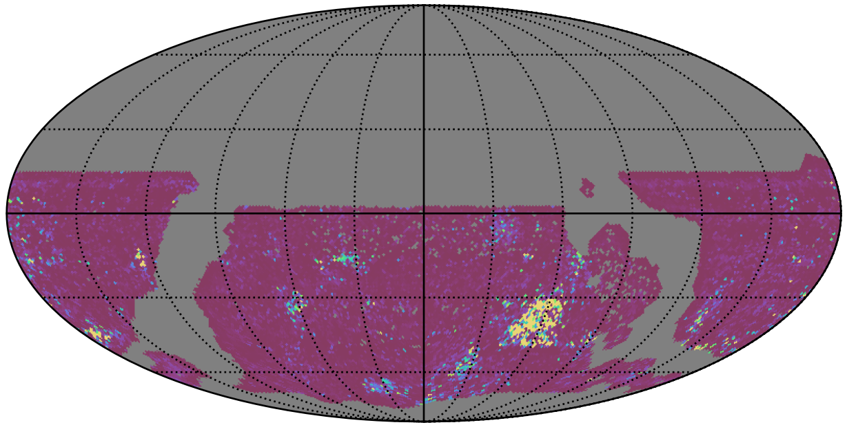
too_elab_r16_d3_gz_v3.4_10yrs WFD g band: 75th Percentile Intranight Timespan
