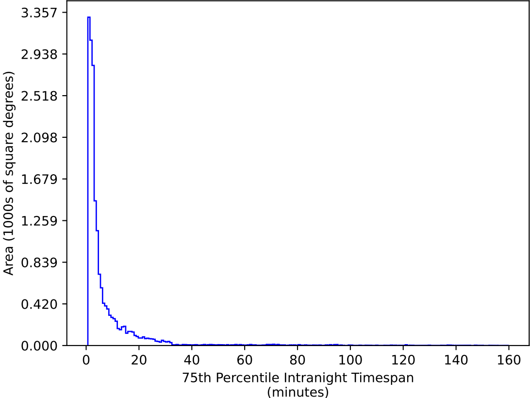
too_elab_r16_d3_gz_v3.4_10yrs WFD g band: 75th Percentile Intranight Timespan
