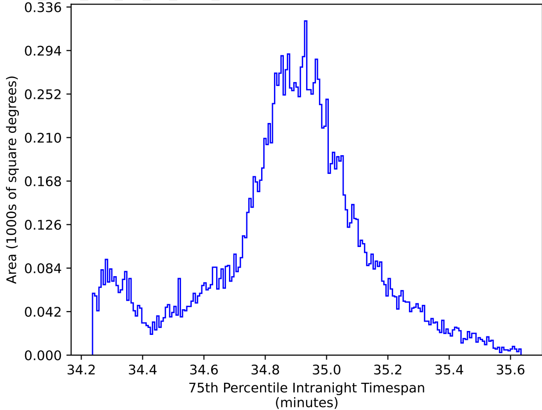
too_elab_r16_d3_gz_v3.4_10yrs WFD: 75th Percentile Intranight Timespan
