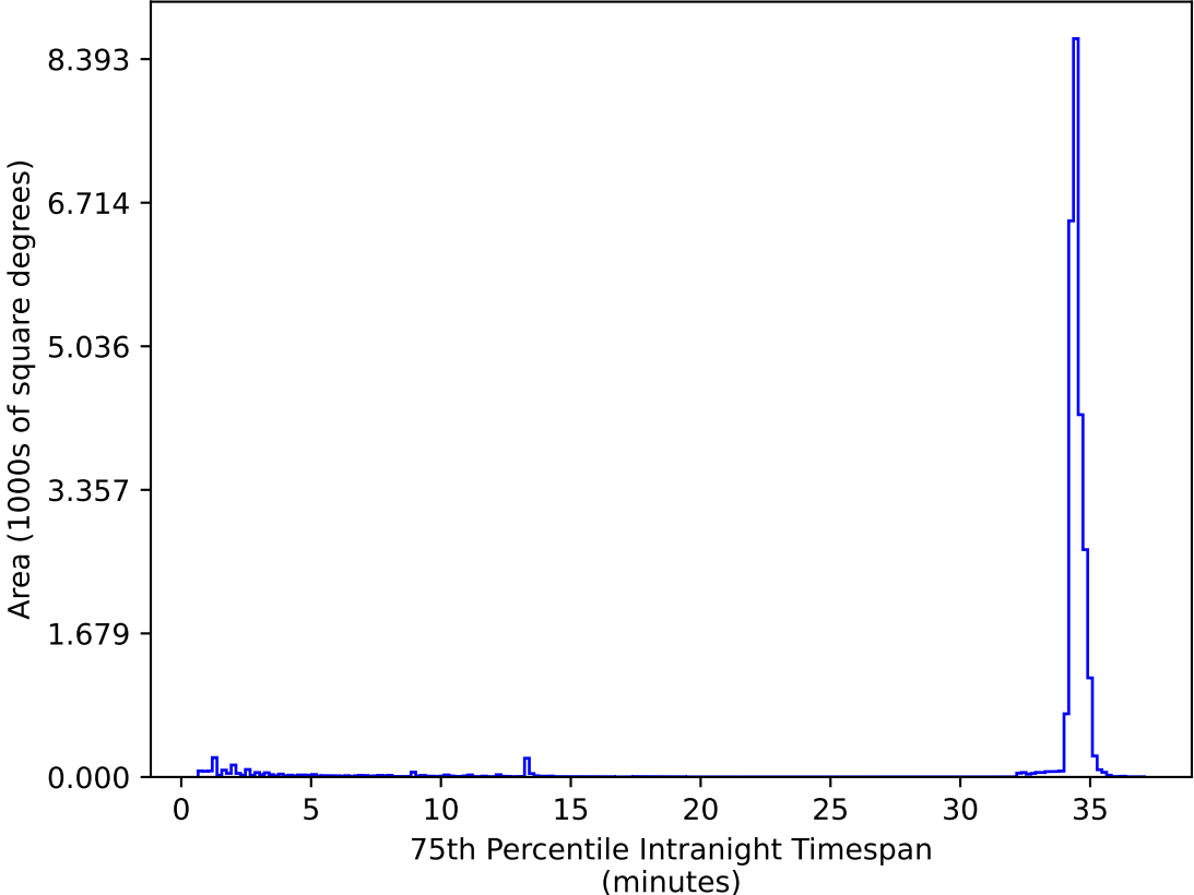
too_elab_r16_d3_gz_v3.4_10yrs All sky zy bands: 75th Percentile Intranight Timespan
