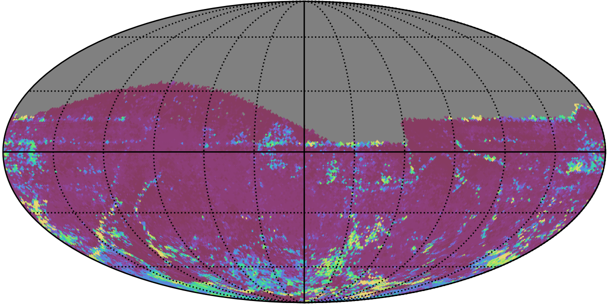
too_elab_r16_d3_gz_v3.4_10yrs All sky z band: 75th Percentile Intranight Timespan
