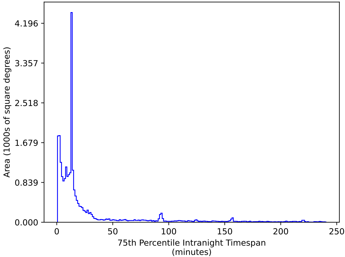
too_elab_r16_d3_gz_v3.4_10yrs All sky z band: 75th Percentile Intranight Timespan
