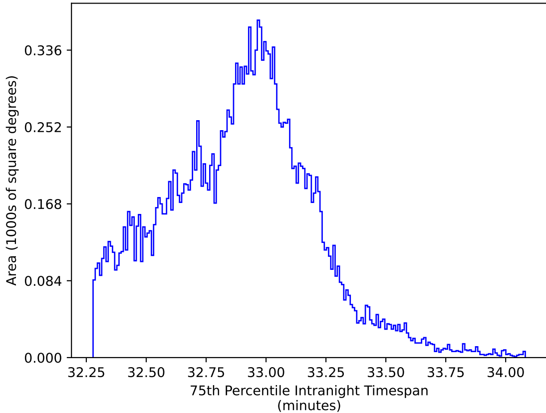
too_elab_r16_d3_gz_v3.4_10yrs All sky y band: 75th Percentile Intranight Timespan
