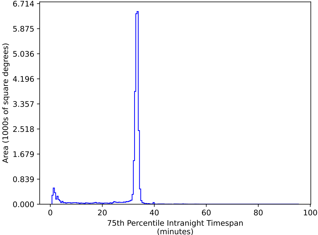
too_elab_r16_d3_gz_v3.4_10yrs All sky ug bands: 75th Percentile Intranight Timespan
