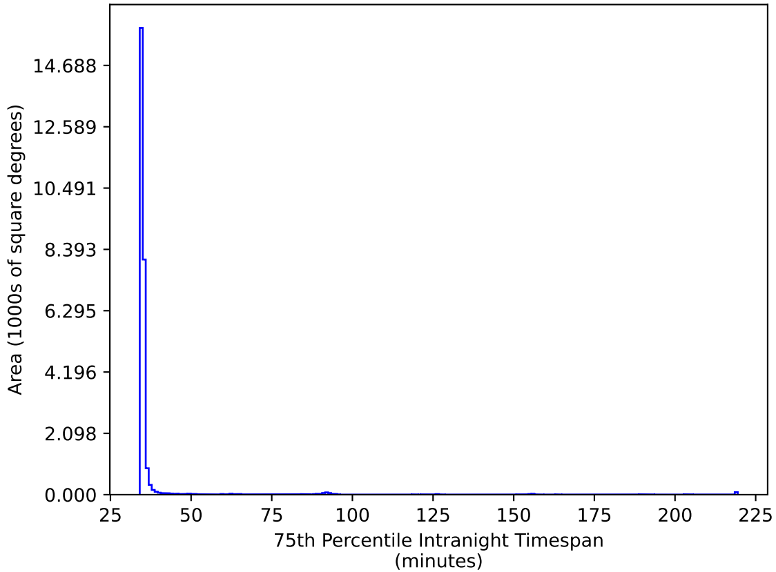
too_elab_r16_d3_gz_v3.4_10yrs All sky ri bands: 75th Percentile Intranight Timespan
