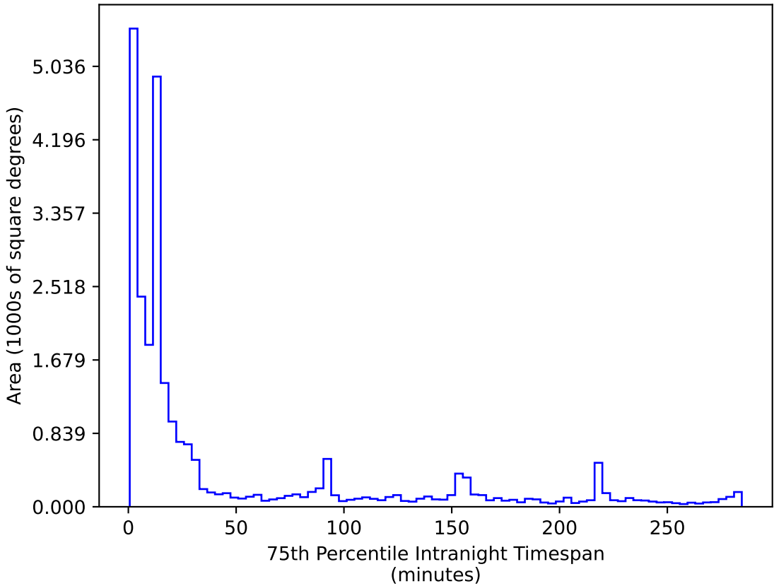
too_elab_r16_d3_gz_v3.4_10yrs All sky r band: 75th Percentile Intranight Timespan
