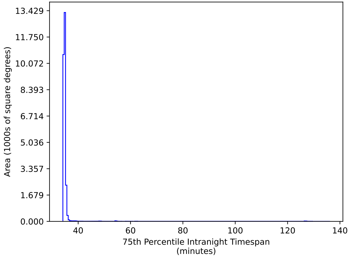
too_elab_r16_d3_gz_v3.4_10yrs All sky iz bands: 75th Percentile Intranight Timespan
