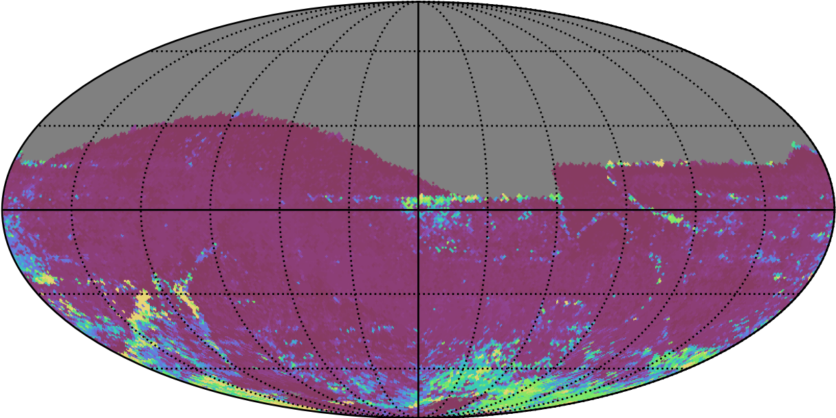
too_elab_r16_d3_gz_v3.4_10yrs All sky i band: 75th Percentile Intranight Timespan
