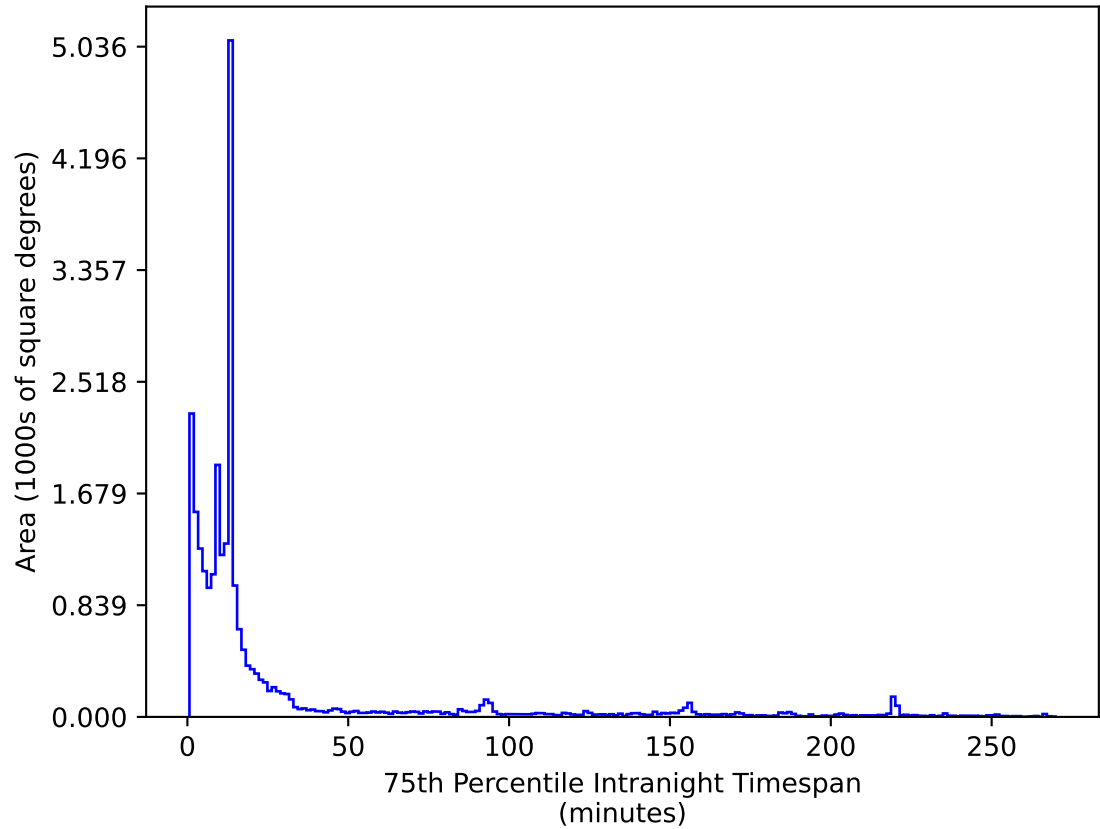
too_elab_r16_d3_gz_v3.4_10yrs All sky i band: 75th Percentile Intranight Timespan
