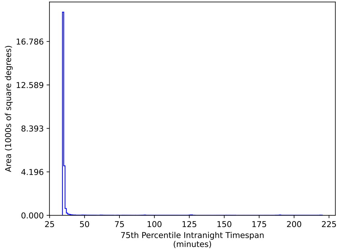
too_elab_r16_d3_gz_v3.4_10yrs All sky gr bands: 75th Percentile Intranight Timespan
