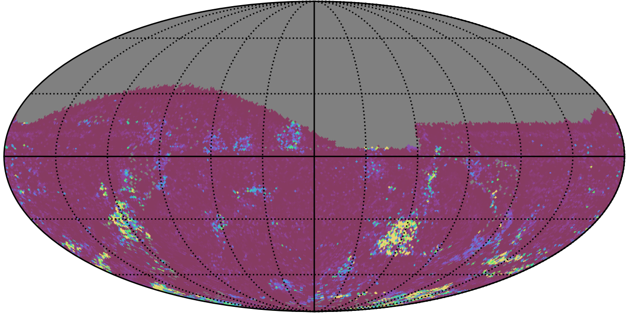
too_elab_r16_d3_gz_v3.4_10yrs All sky g band: 75th Percentile Intranight Timespan
