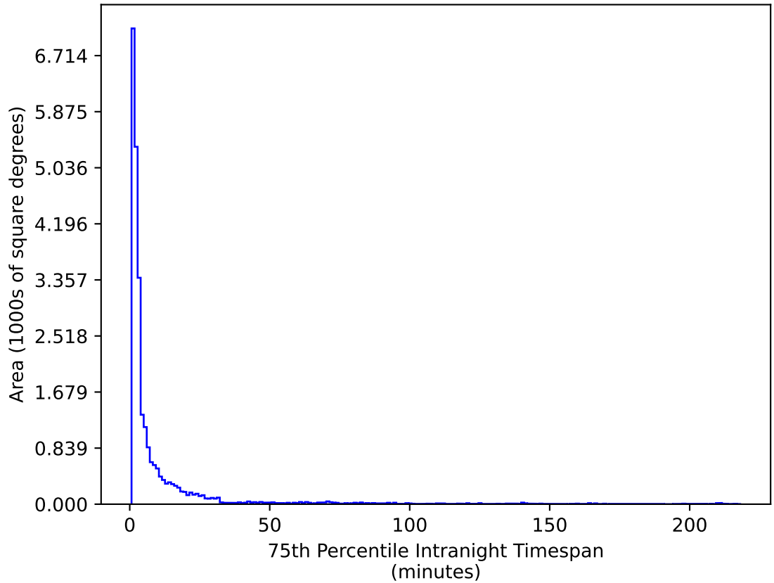
too_elab_r16_d3_gz_v3.4_10yrs All sky g band: 75th Percentile Intranight Timespan
