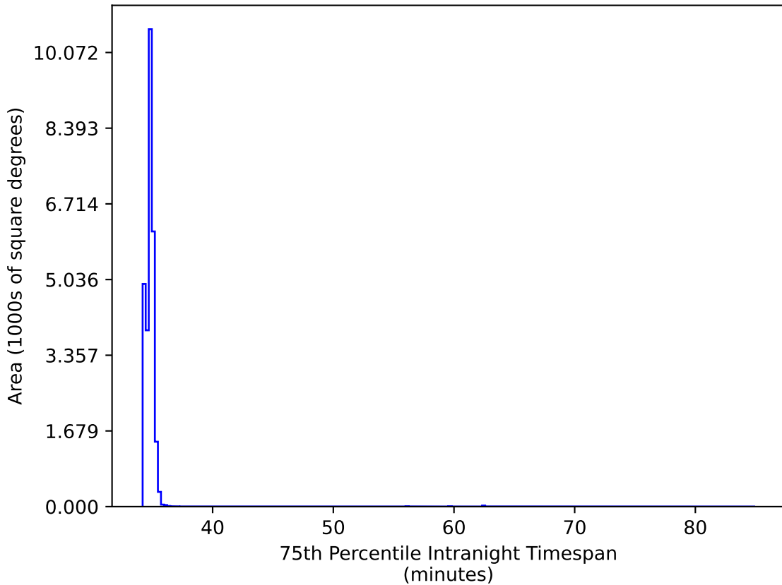
too_elab_r16_d3_gz_v3.4_10yrs All sky: 75th Percentile Intranight Timespan
