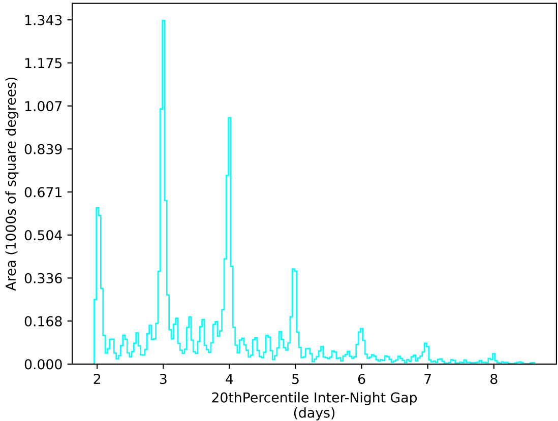
too_elab_r16_d3_gz_v3.4_10yrs WFD u band: 20thPercentile Inter-Night Gap
