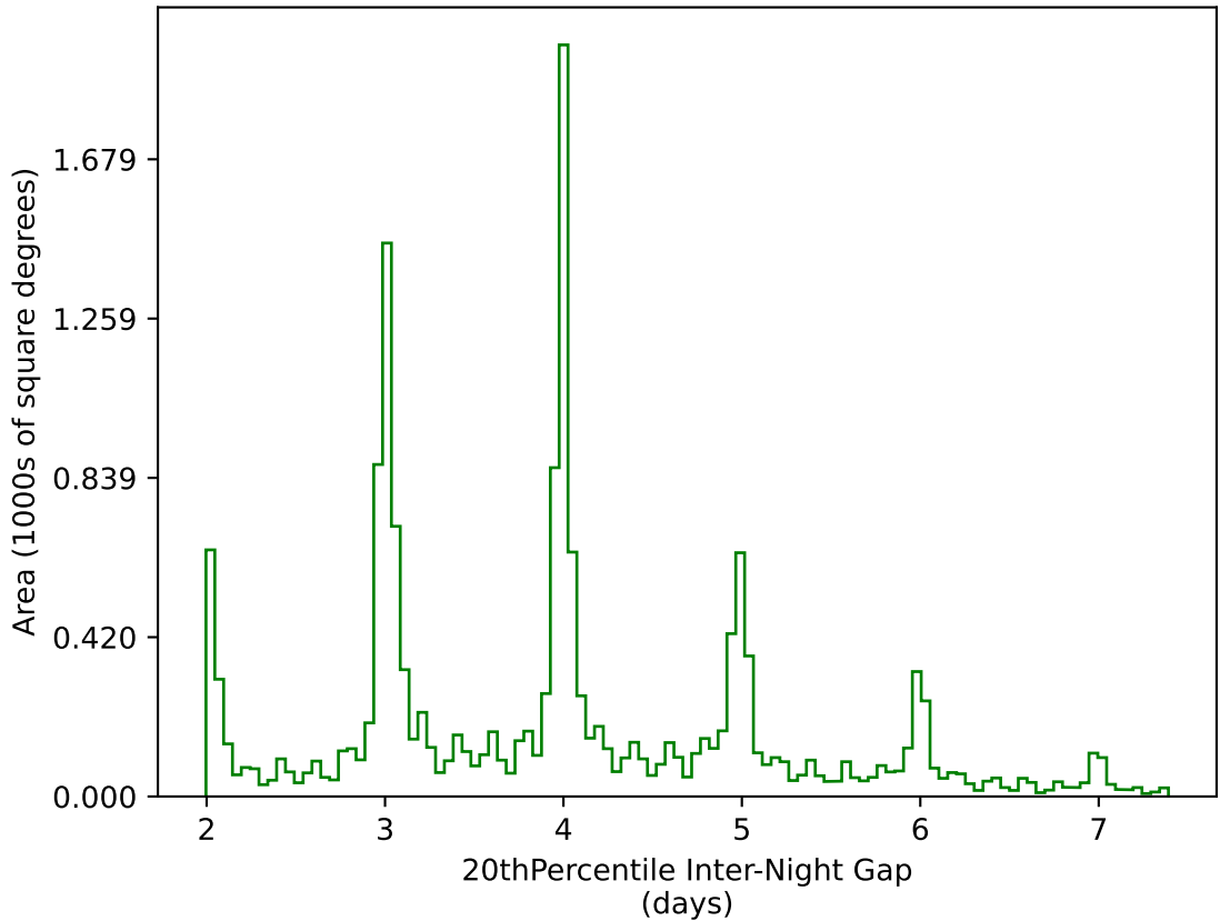
too_elab_r16_d3_gz_v3.4_10yrs WFD g band: 20thPercentile Inter-Night Gap
