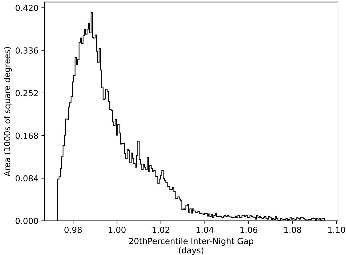
too_elab_r16_d3_gz_v3.4_10yrs WFD all bands: 20thPercentile Inter-Night Gap
