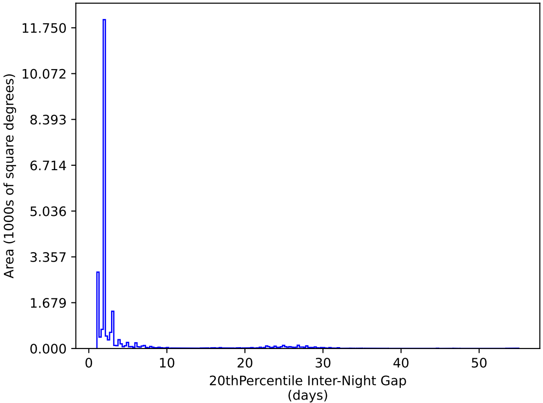
too_elab_r16_d3_gz_v3.4_10yrs All sky y band: 20thPercentile Inter-Night Gap
