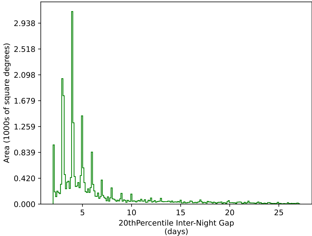
too_elab_r16_d3_gz_v3.4_10yrs All sky g band: 20thPercentile Inter-Night Gap
