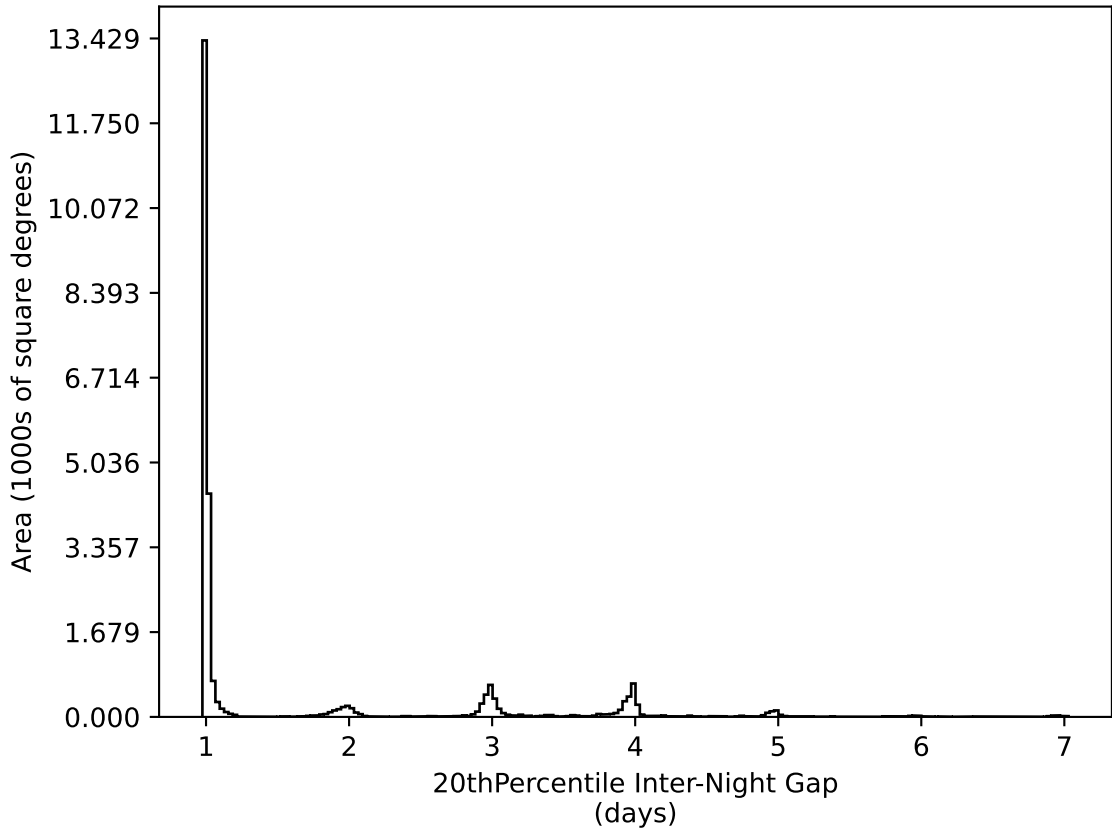
too_elab_r16_d3_gz_v3.4_10yrs All sky all bands: 20thPercentile Inter-Night Gap
