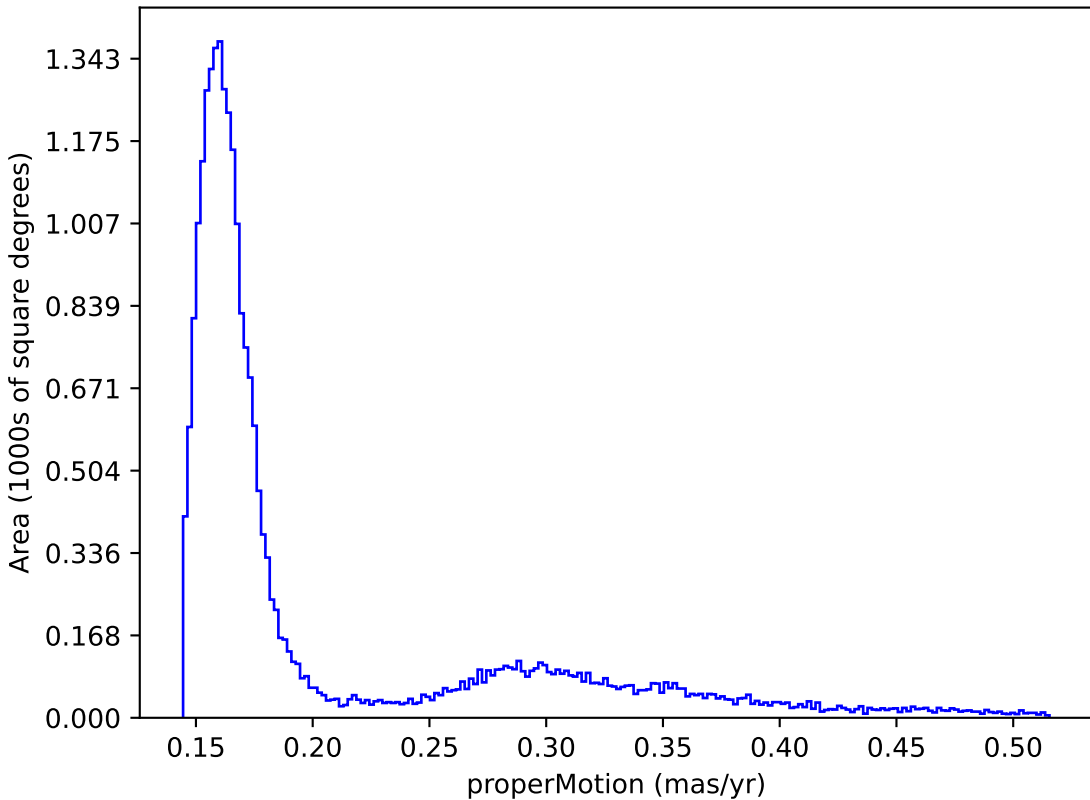
too_elab_r16_d3_gz_v3.4_10yrs : properMotion
