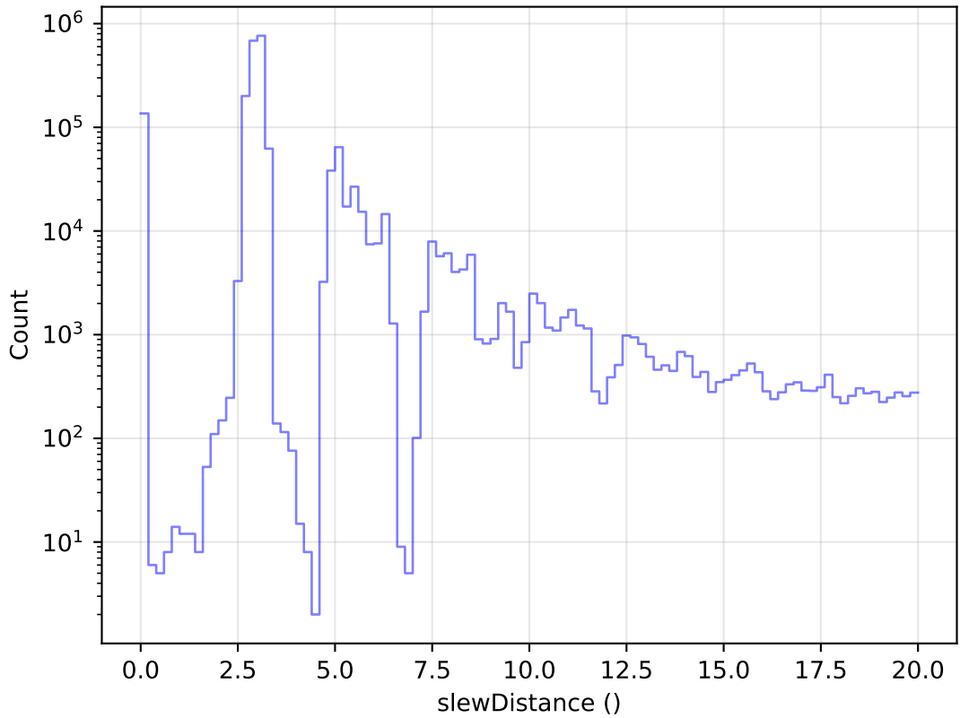
too_elab_r16_d3_gz_v3.4_10yrs All visits: Zoom Slew Distance Histogram
