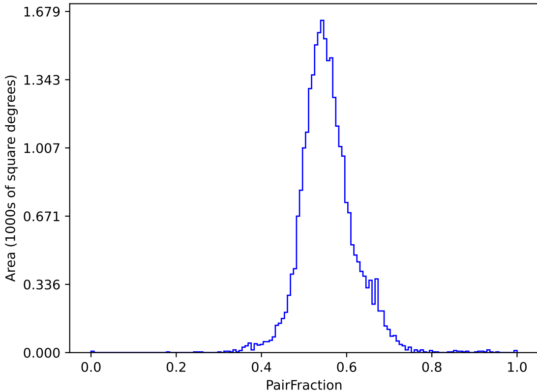
too_elab_r16_d3_gz_v3.4_10yrs (g or r or i): PairFraction
