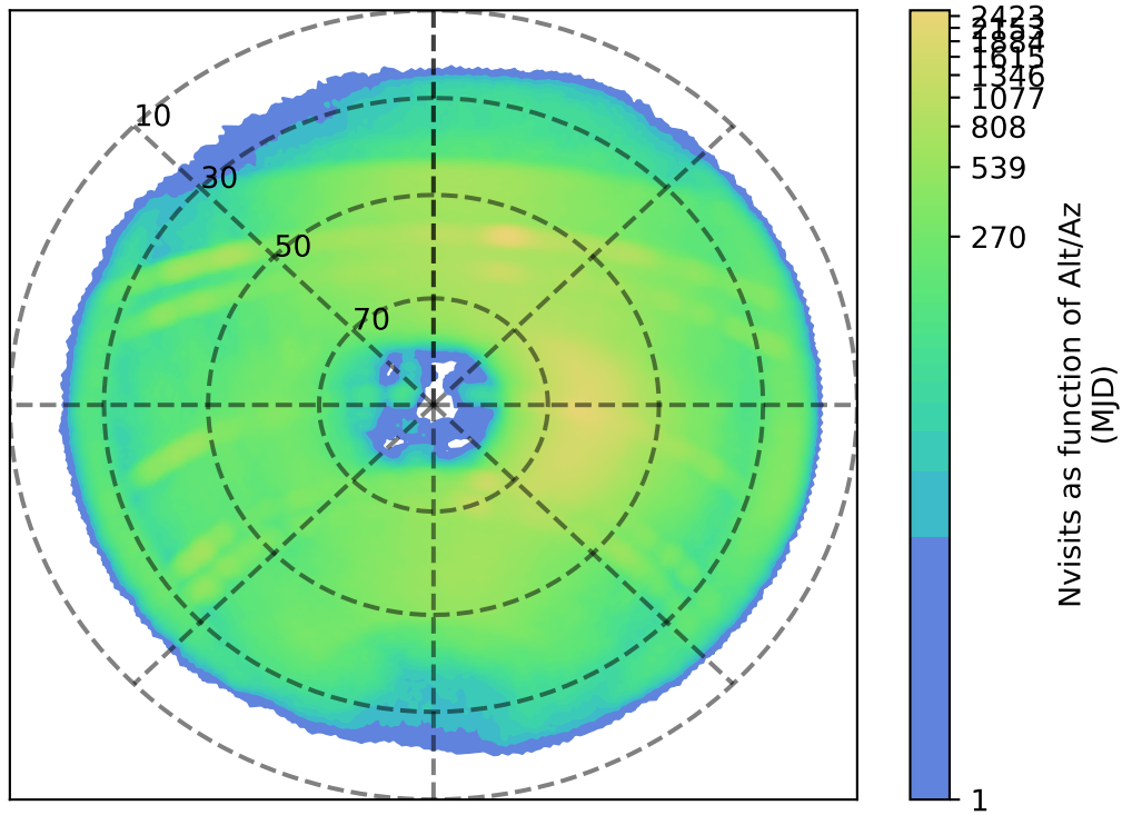
too_elab_r16_d3_gz_v3.4_10yrs z: Nvisits as function of Alt/Az
