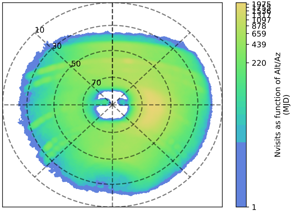
too_elab_r16_d3_gz_v3.4_10yrs y: Nvisits as function of Alt/Az
