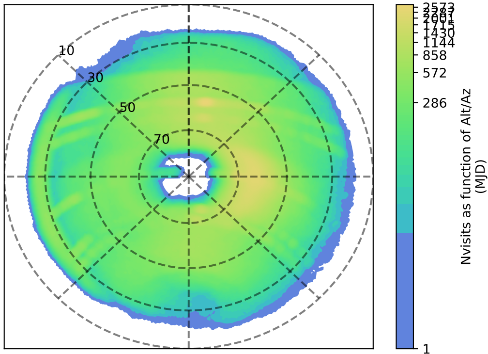
too_elab_r16_d3_gz_v3.4_10yrs r: Nvisits as function of Alt/Az
