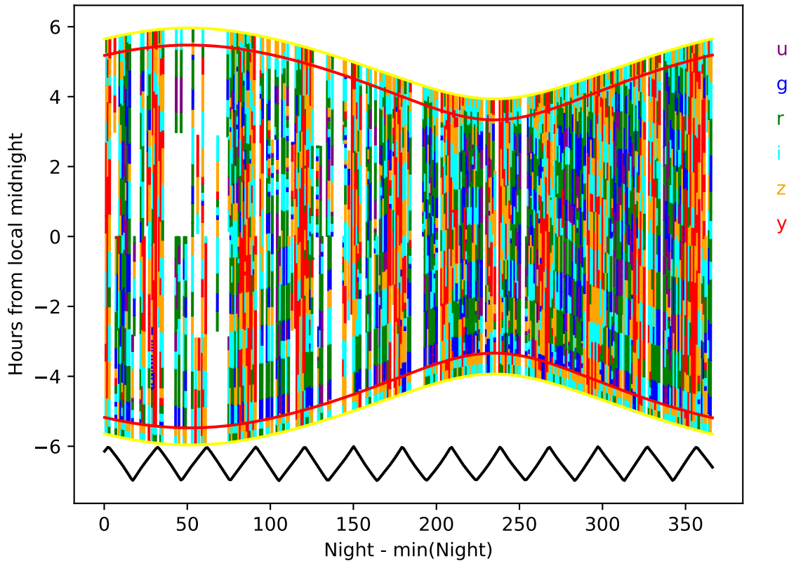
too_elab_r16_d3_gz_v3.4_10yrs year 9-10: Hourglass
