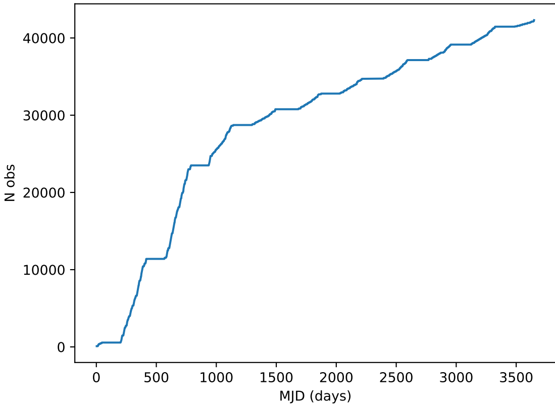
too_elab_r16_d3_gz_v3.4_10yrs note like DD:COSMOS%: Cumulative
