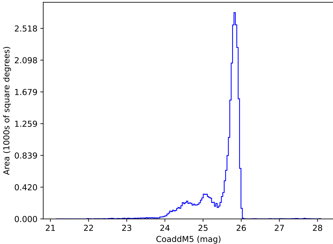
too_elab_r16_d3_gz_v3.4_10yrs z: CoaddM5
