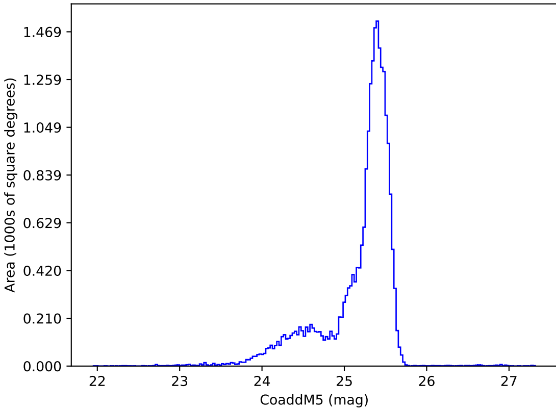
too_elab_r16_d3_gz_v3.4_10yrs u: CoaddM5
