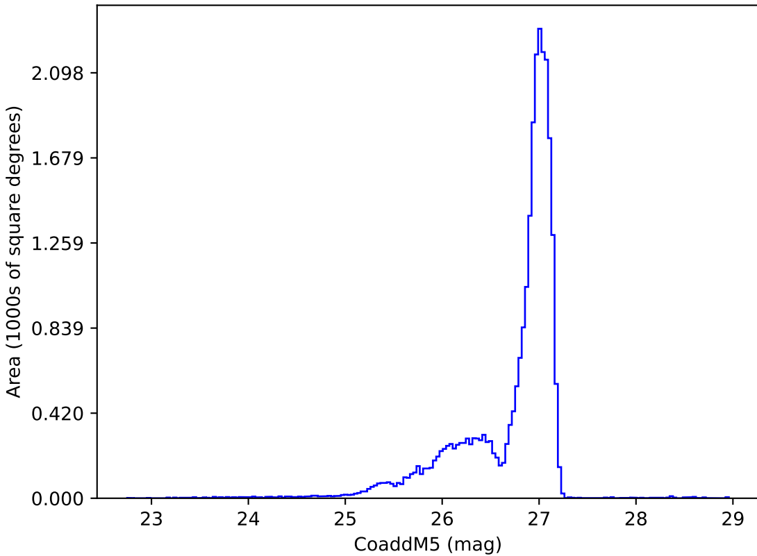
too_elab_r16_d3_gz_v3.4_10yrs r: CoaddM5
