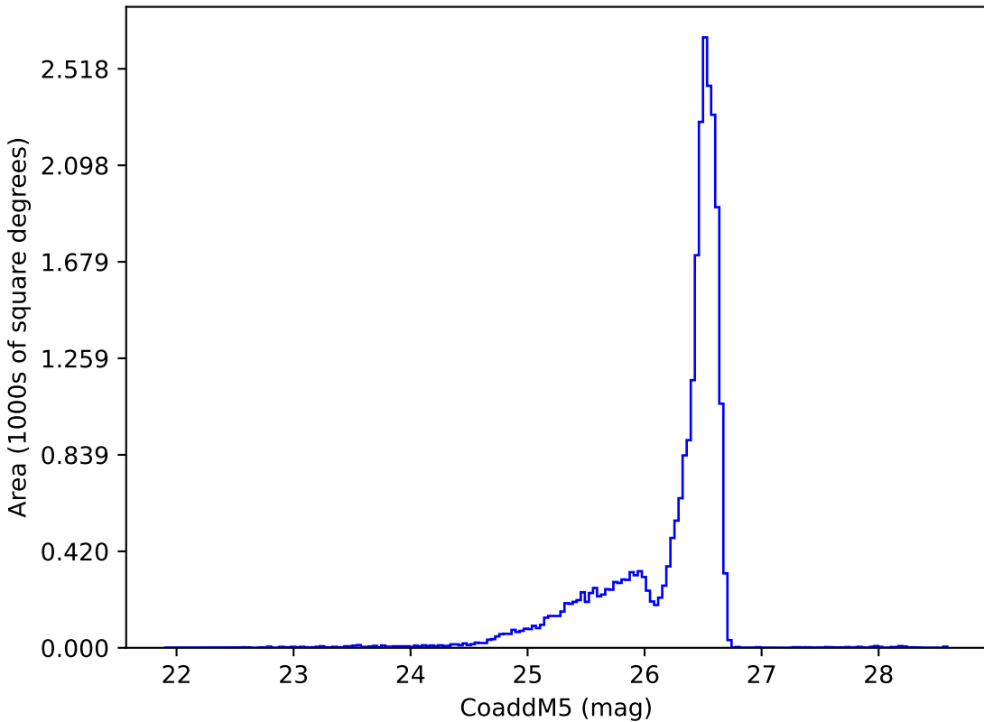
too_elab_r16_d3_gz_v3.4_10yrs i: CoaddM5
