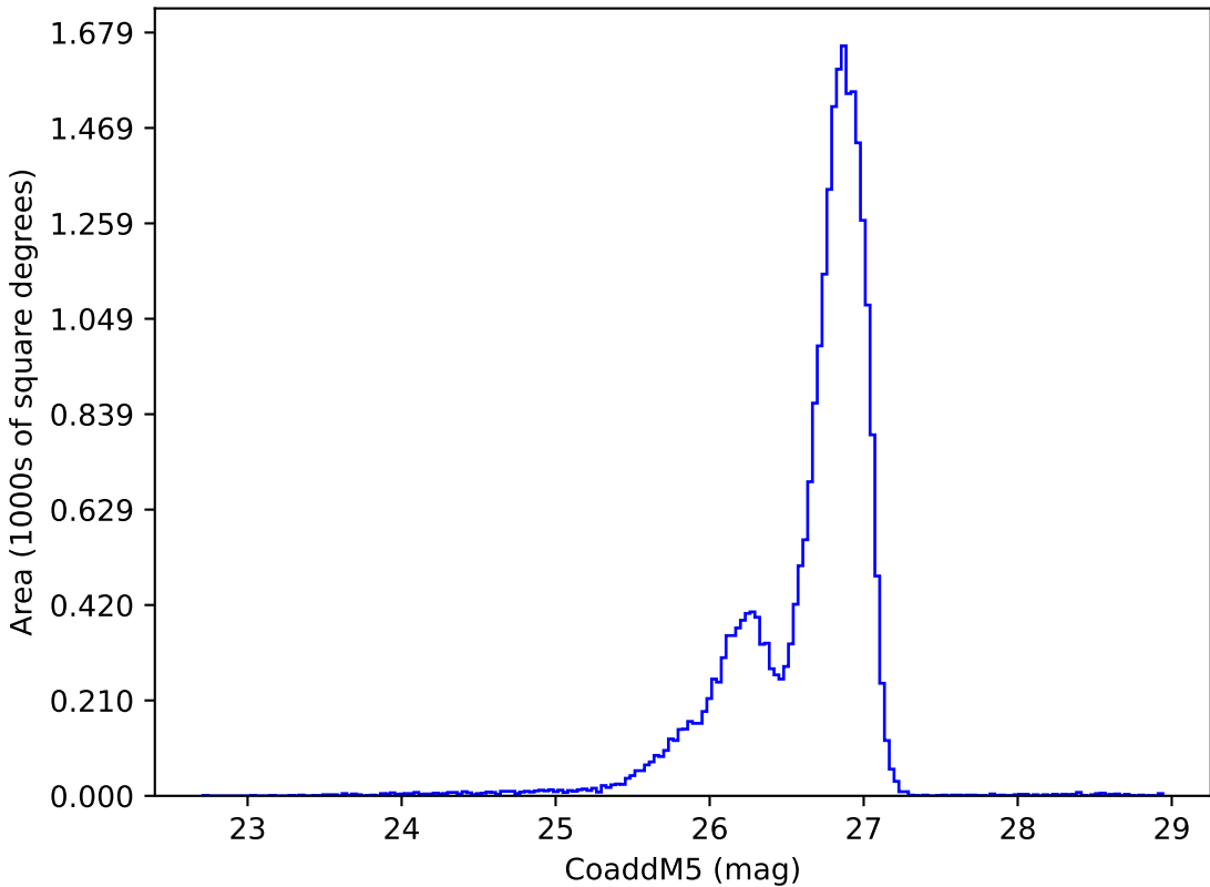
too_elab_r16_d3_gz_v3.4_10yrs g: CoaddM5
