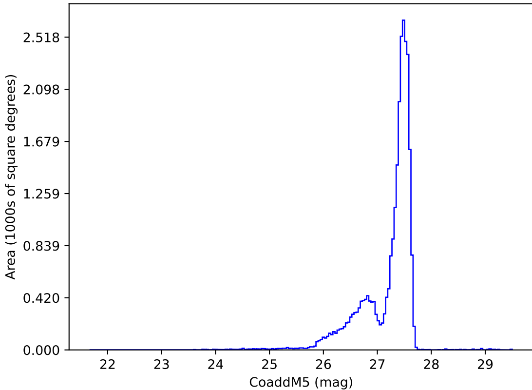
too_elab_r16_d3_gz_v3.4_10yrs : CoaddM5
