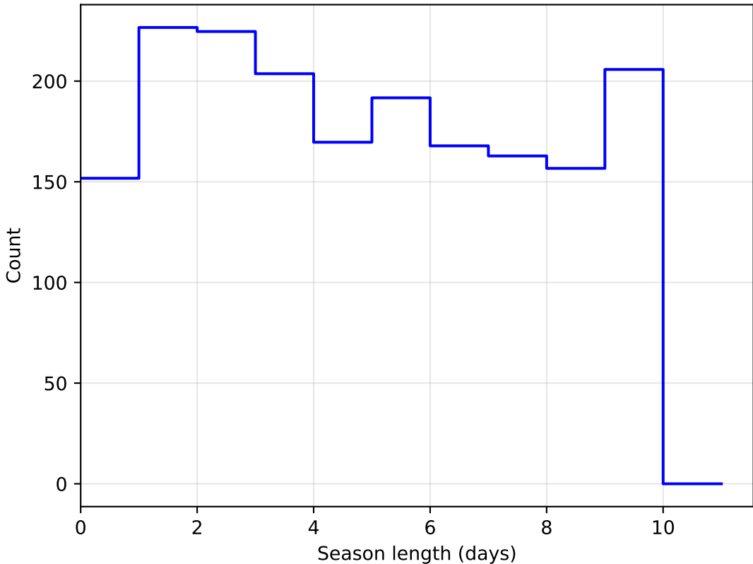
too_elab_r16_d3_gz_v3.4_10yrs DD:WFD all bands: SeasonLength
