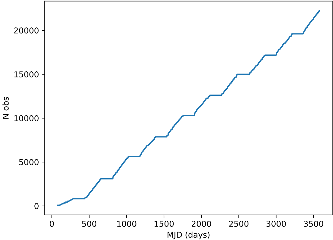
too_elab_r16_d3_gz_v3.4_10yrs all bands: DD:XMM_LSS Cumulative NVisits
