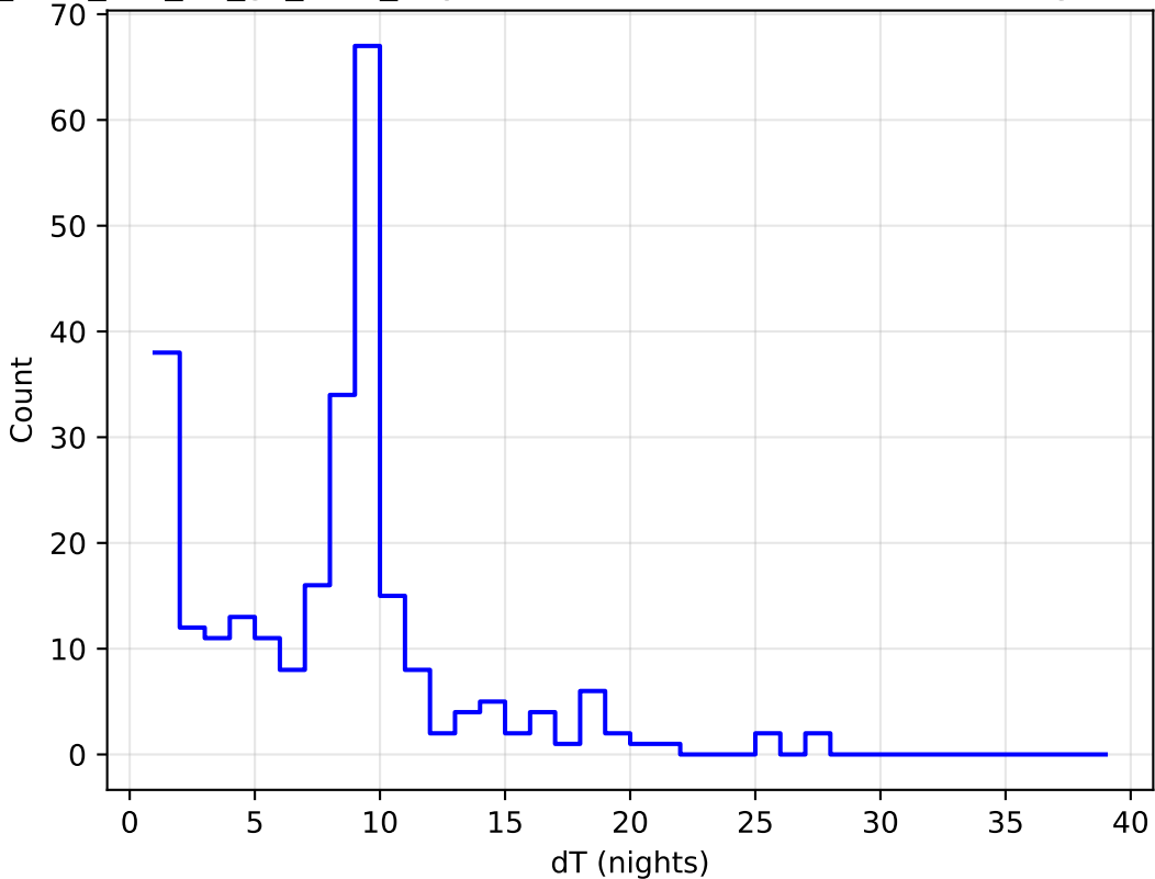
too_elab_r16_d3_gz_v3.4_10yrs all bands: DD:ELAISS1 Delta Nights Histogram
