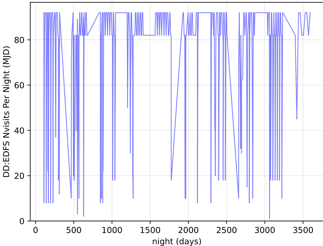
too_elab_r16_d3_gz_v3.4_10yrs all bands: DD:EDFS Nvisits Per Night
