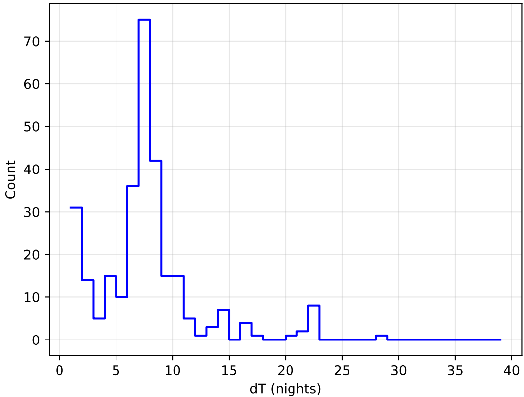
too_elab_r16_d3_gz_v3.4_10yrs all bands: DD:EDFS Delta Nights Histogram
