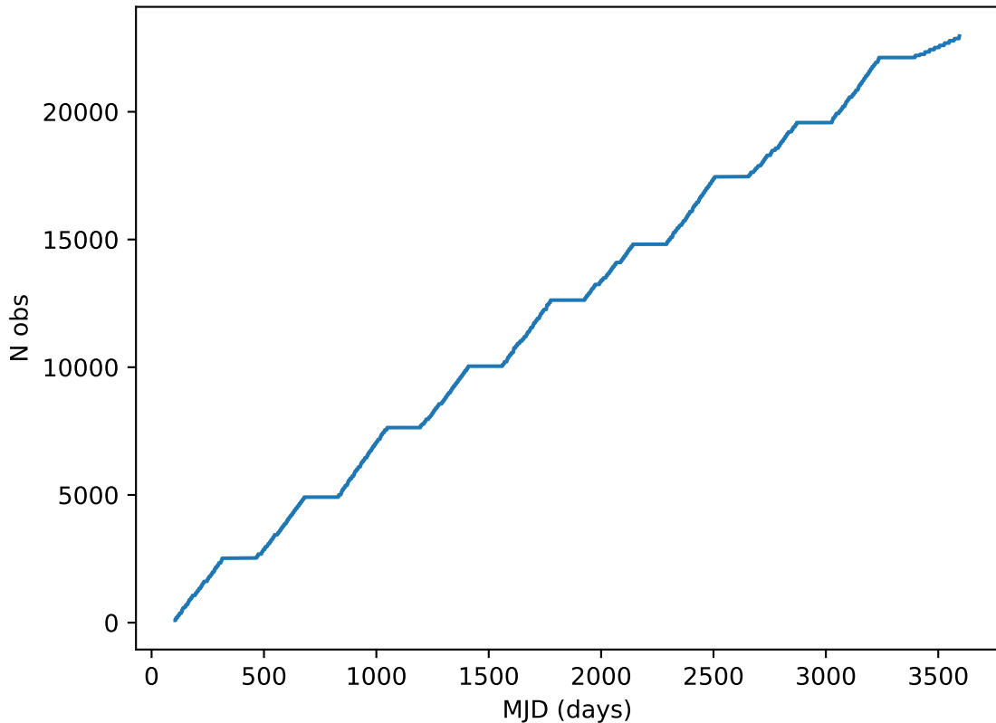
too_elab_r16_d3_gz_v3.4_10yrs all bands: DD:EDFS Cumulative NVisits
