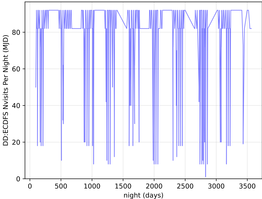
too_elab_r16_d3_gz_v3.4_10yrs all bands: DD:ECDFS Nvisits Per Night
