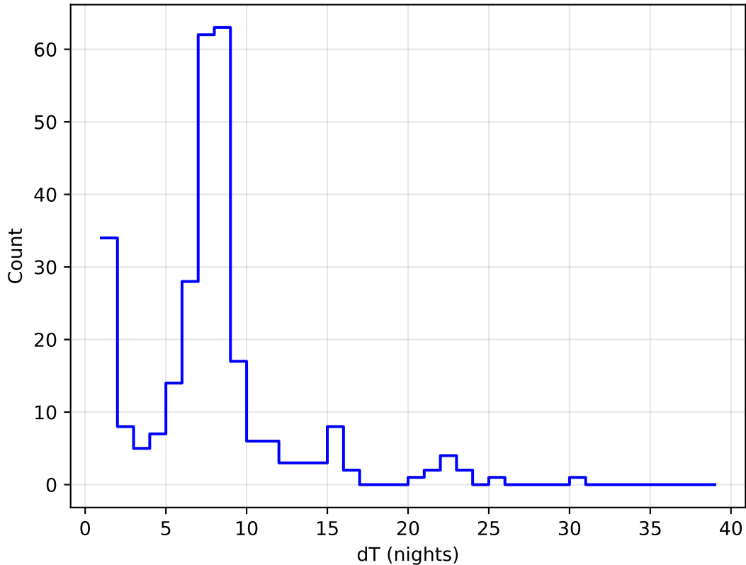
too_elab_r16_d3_gz_v3.4_10yrs all bands: DD:ECDFS Delta Nights Histogram
