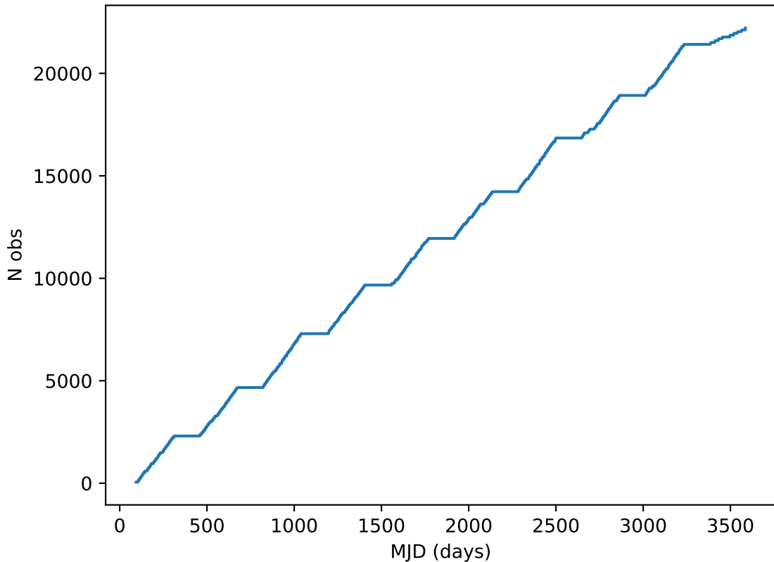
too_elab_r16_d3_gz_v3.4_10yrs all bands: DD:ECDFS Cumulative NVisits
