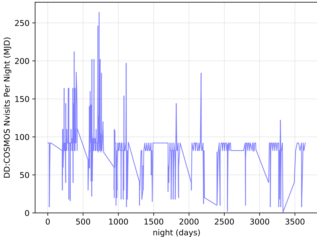
too_elab_r16_d3_gz_v3.4_10yrs all bands: DD: COSMOS Nvisits Per Night
