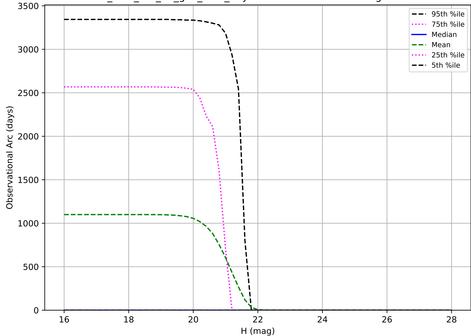
too_elab_r16_d3_griz_v3.4_10yrs: Observational Arc Length Vatira
