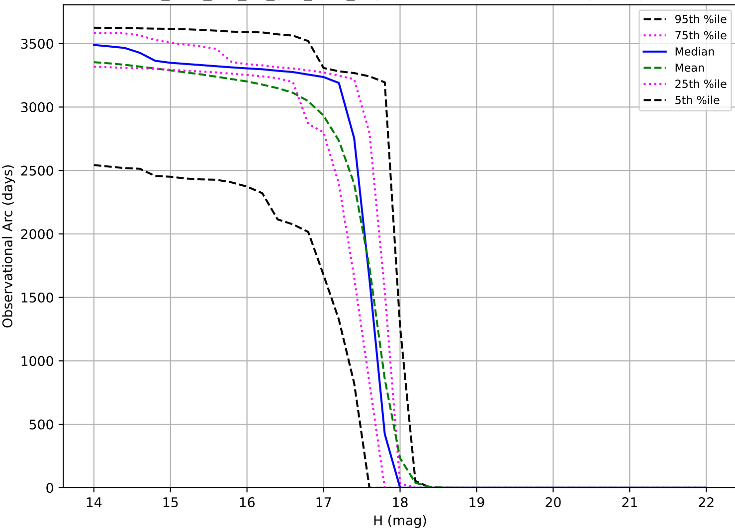
too_elab_r16_d3_griz_v3.4_10yrs: Observational Arc Length Trojan
